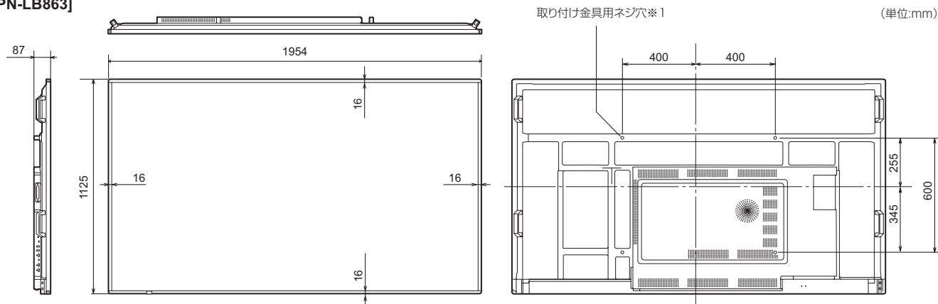
[PN-LB863]
