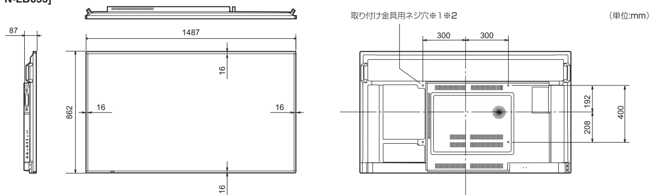
[PN-LB653]
