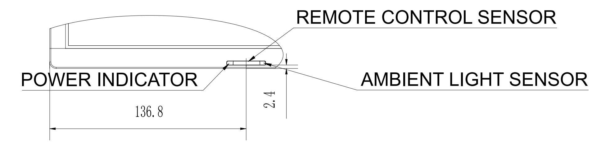
DETAIL C
