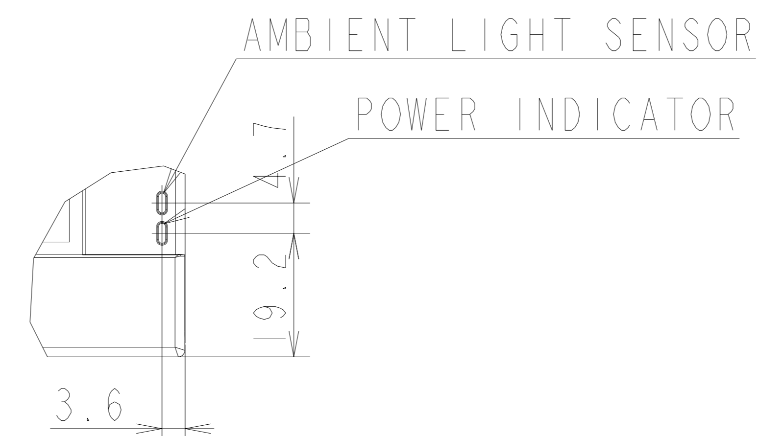
DETAIL A
